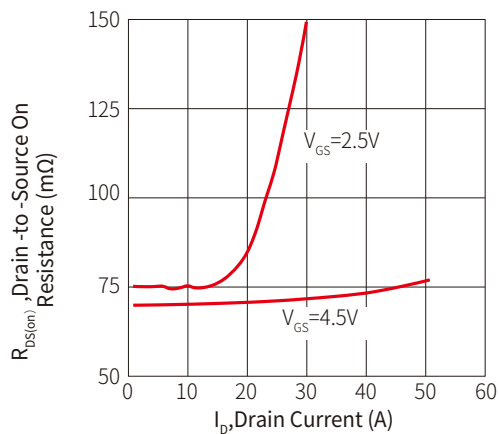
Figure 11: Typical On-Resistance Vs. Drain Current
