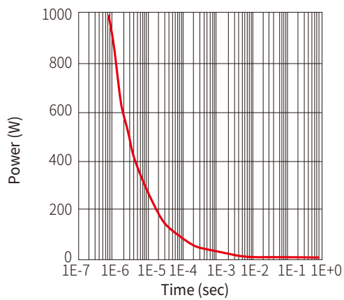
Figure 13: Typical Power Vs. Time
