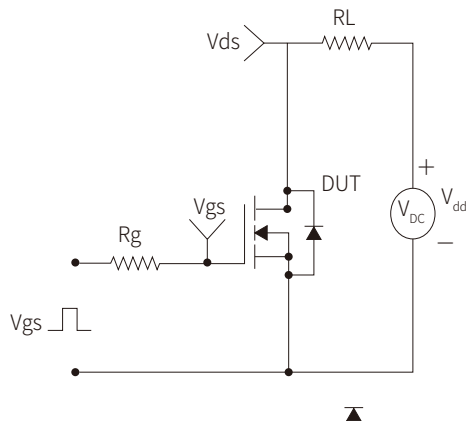
Figure 13: Resistive Switching Test Circuit & Waveforms
