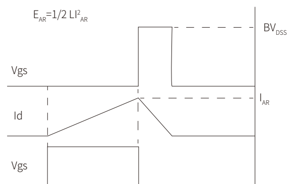
Figure 14: Unclamped Inductive Switching (UIS) Test Circuit & Waveforms
