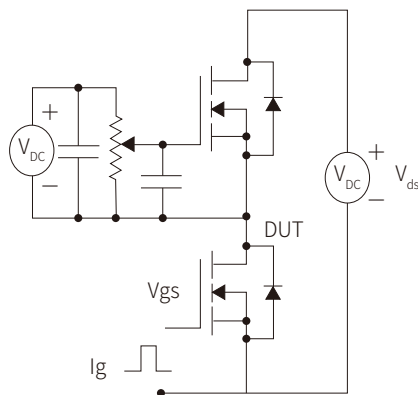
Figure 12: Gate Charge Test Circuit & Waveform
