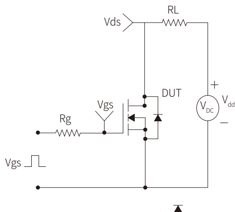
Figure 13: Resistive Switching Test Circuit & Waveforms
