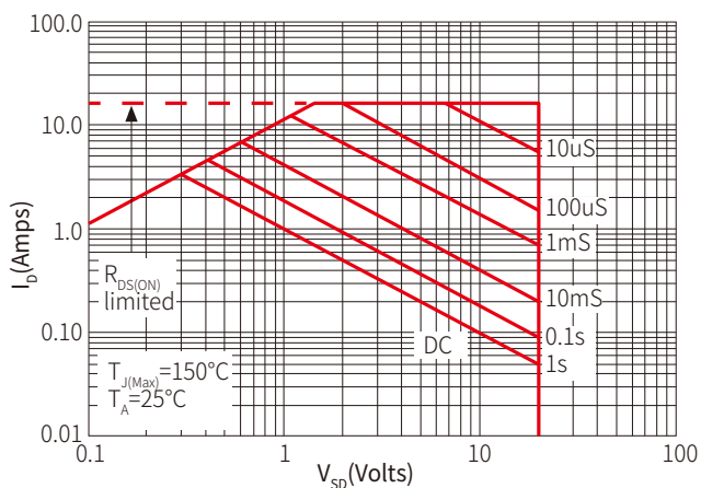
Figure 9: Maximum Forward Biased Safe Operating Are
