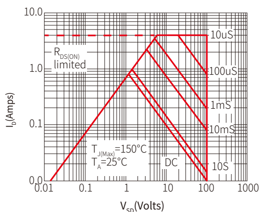
Figure 9: Maximum Forward Biased Safe Operating Are
