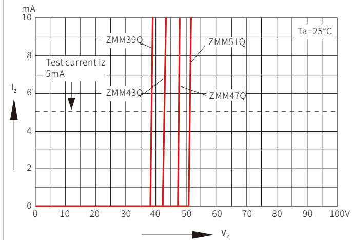
Breakdown characteristics
